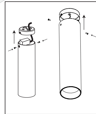
Tube 55 Surface/Superficie
