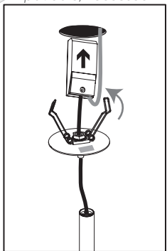
Tube 25 Empotrable/Recessed
